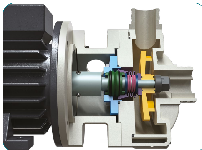
TS = TBELLOWS SEAL
