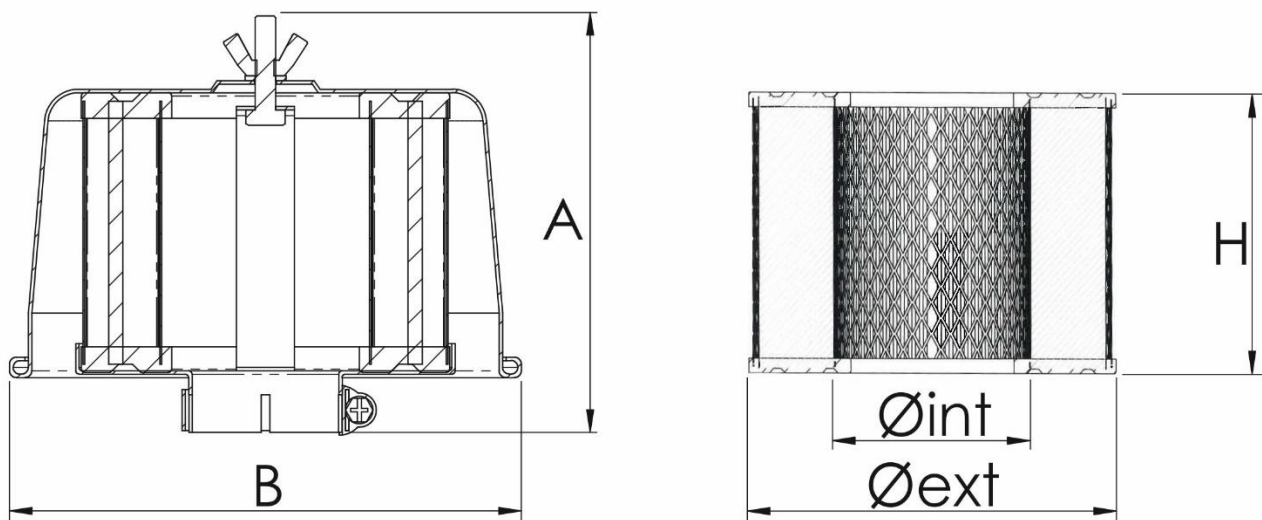
Filter with PVC spool pipe included
