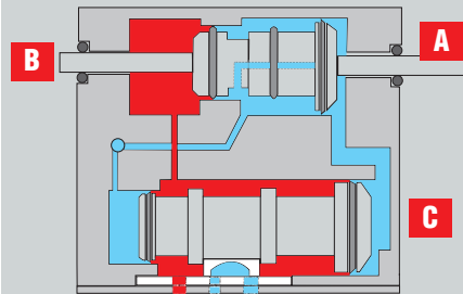
Diaphragm Moving from Left to Right
