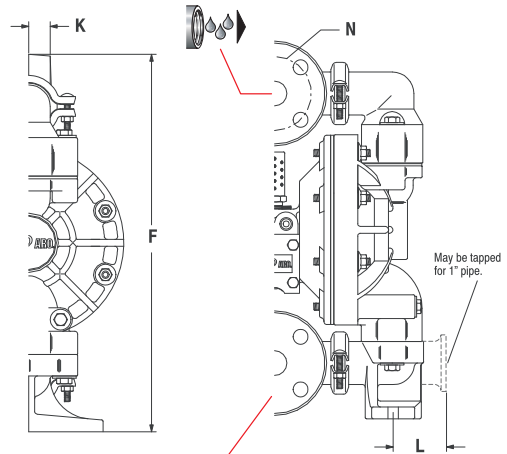
6661X3-X, 6661X4-X, 6661XF-X, 6661XG-X : 1" A.N.S.I./DIN Flange
